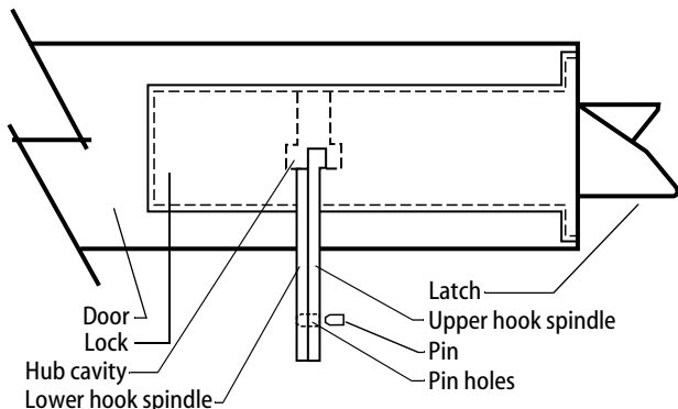
Figure 1—Top, cut-away view of an installed mortise lock case
