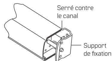
Figure 10 Support de montage
