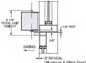
SECTION VIEW
