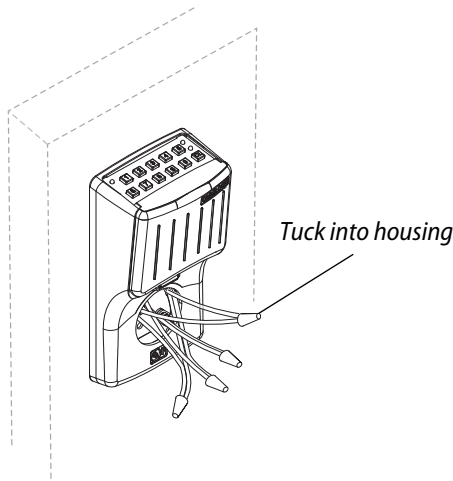
Figure 5 Installing escutcheon
