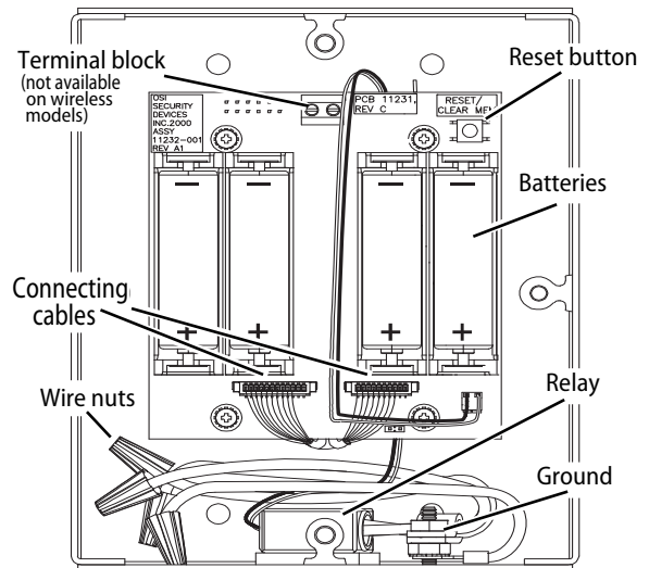
Figure 7 Extreme Weatherized circuit board
