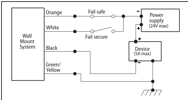
Wire connection diagram
