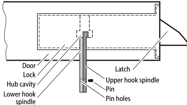
Figure 1 — Top, cut-away view of an installed mortise lock case
