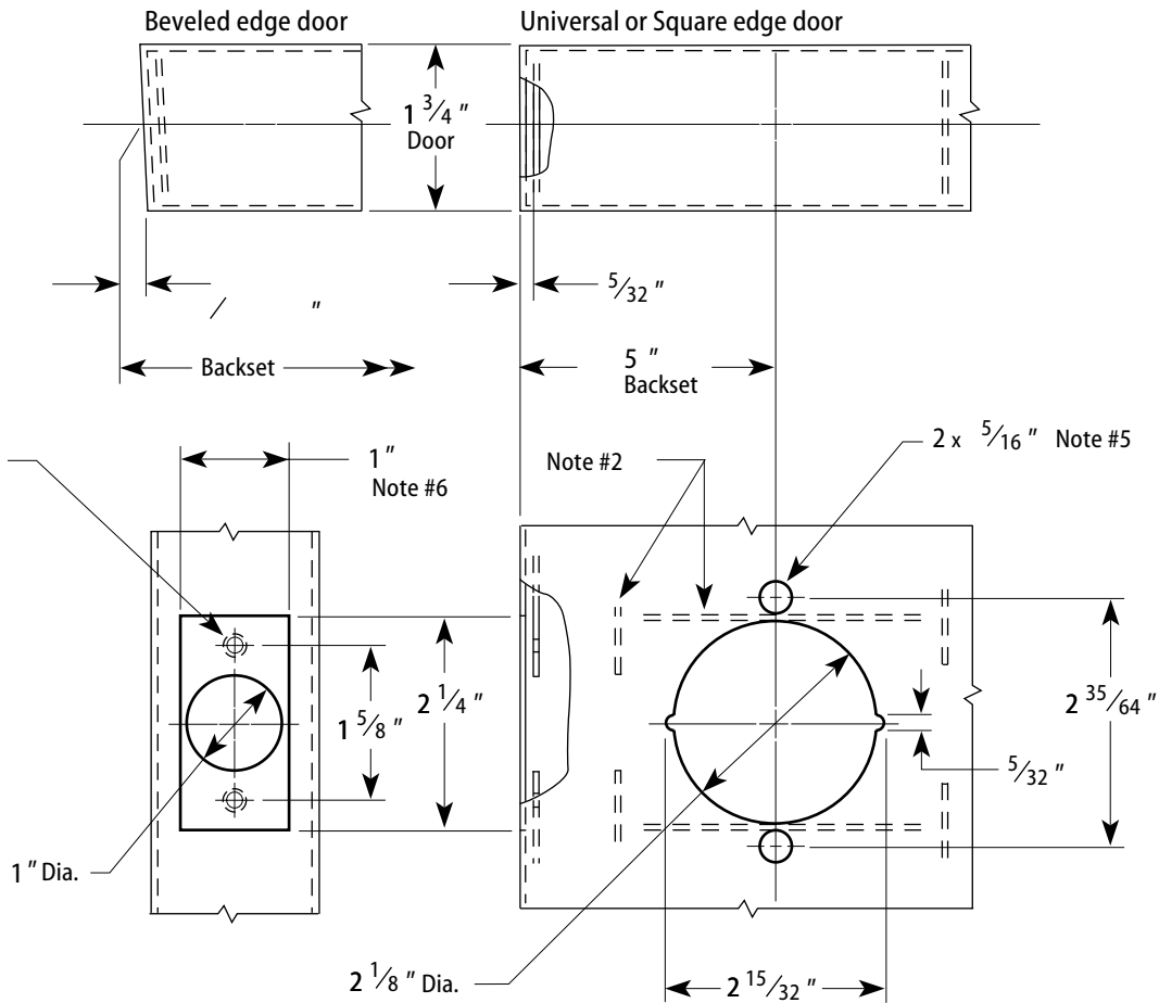
5" Backset Door Preparation
