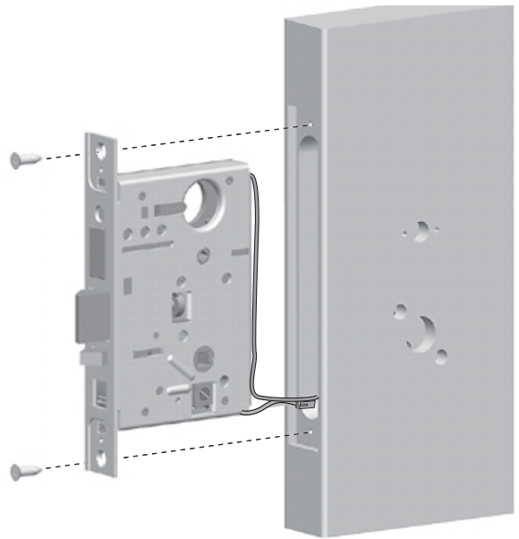
Figure 12 Installing the mortise case
