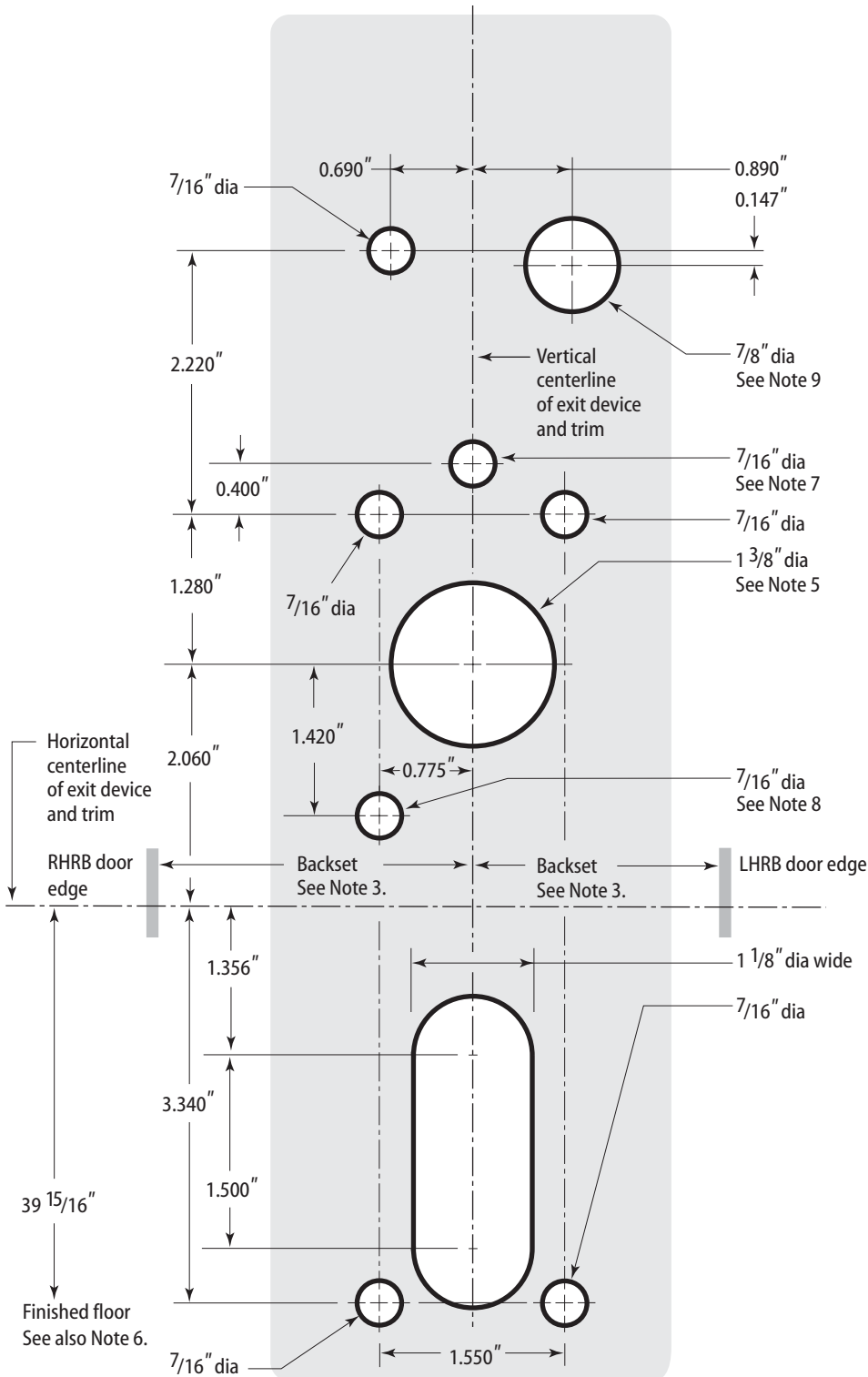
Exit Hardware Trim Escutcheon Footprint (Looking at door from trim side) *Template is not to scale
