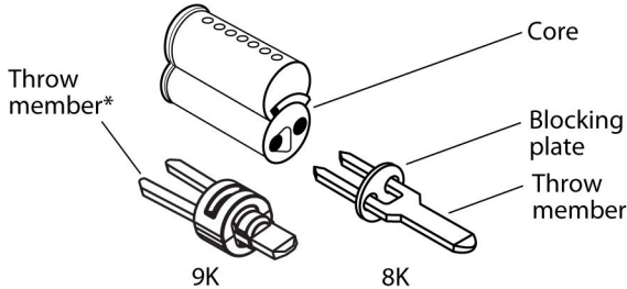
Figure 20a Installing the blocking plate and throw member
