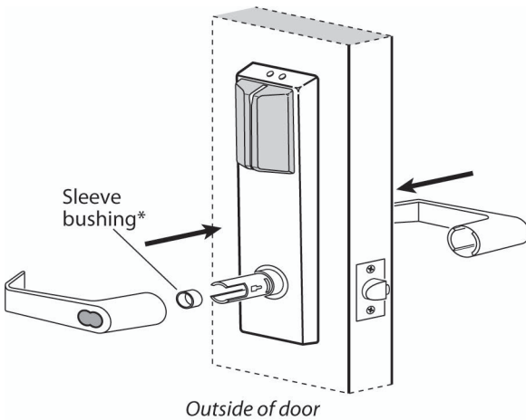
Figure 19 Installing the levers (9K shown)
