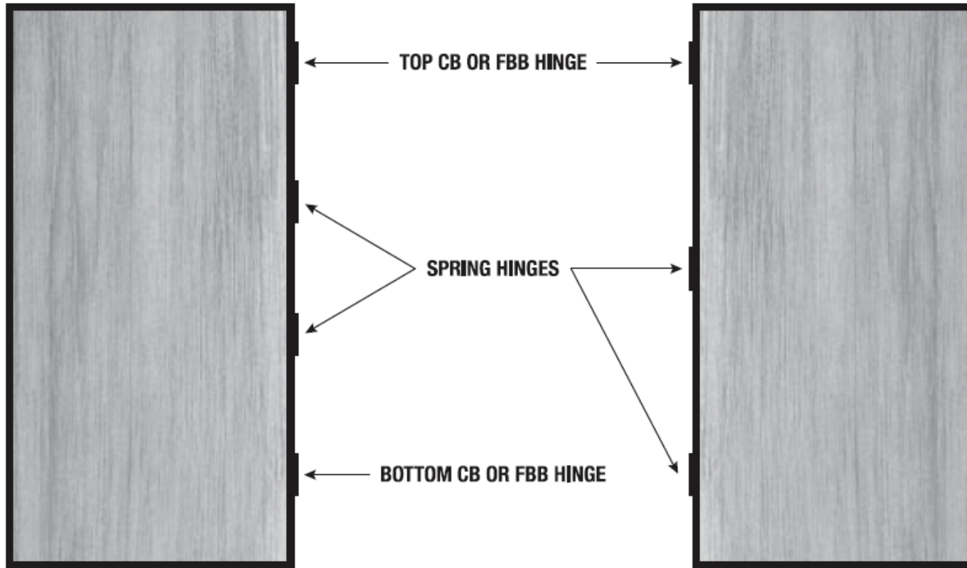
TYPICAL DOOR ELEVATION WHEN USING 4 HINGES
