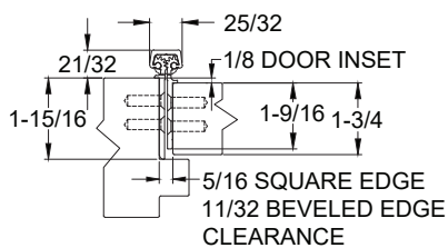
CLOSED POSITION
