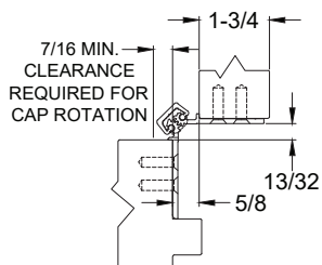
90° OPENING
