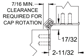
90° OPENING
