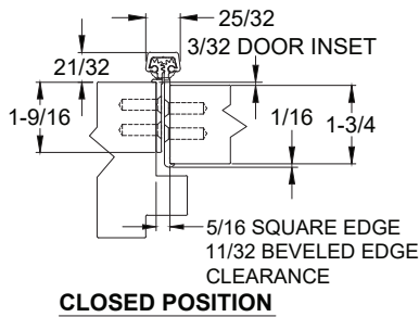
CLOSED POSITION
