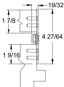
180° OPENING
