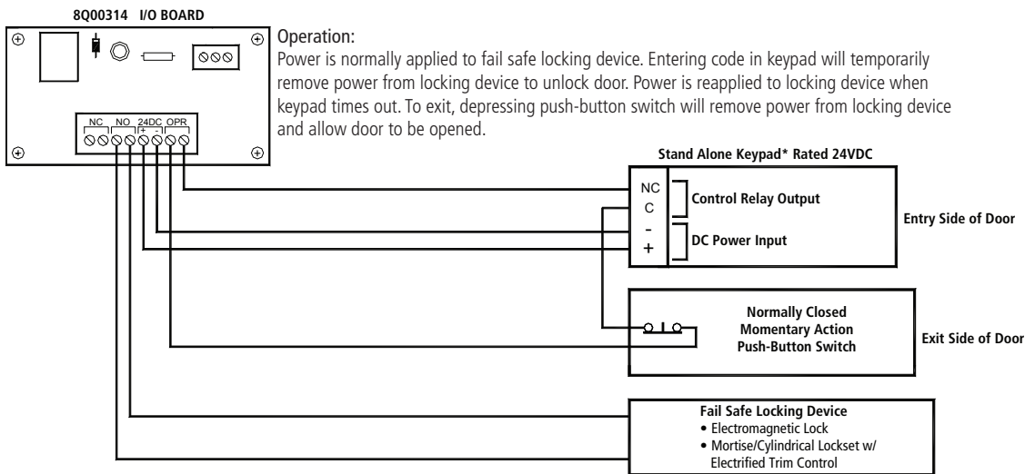
Fig 1: Wire Scheme for a Typical Fail Safe System
