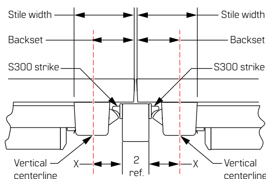
Figure 8 Pair of doors with mullion
