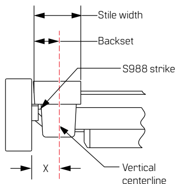
Figure 7 Single aluminum door and frame
