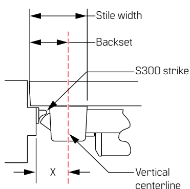
Figure 6 Single hollow metal door
