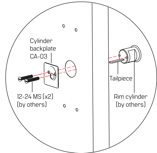
Figure 10 Cylinder only installation
