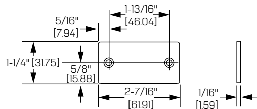
Rub strip S454 (standard)
