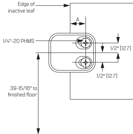
S459 Strike applied to inactive leaf
