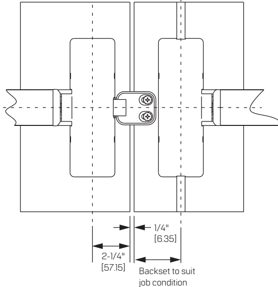
Active leaf rim device Inactive leaf vertical rod device
