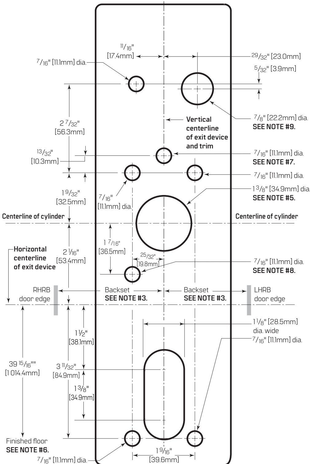
Exit Hardware Trim Escutcheon Footprint (Looking at door from trim side) *Template not to scale
