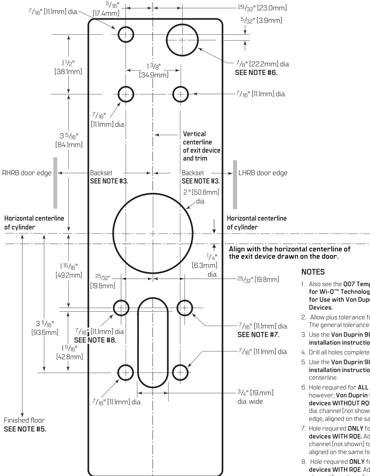
Exit Hardware Trim Escutcheon Footprint [Looking at door from trim side]
