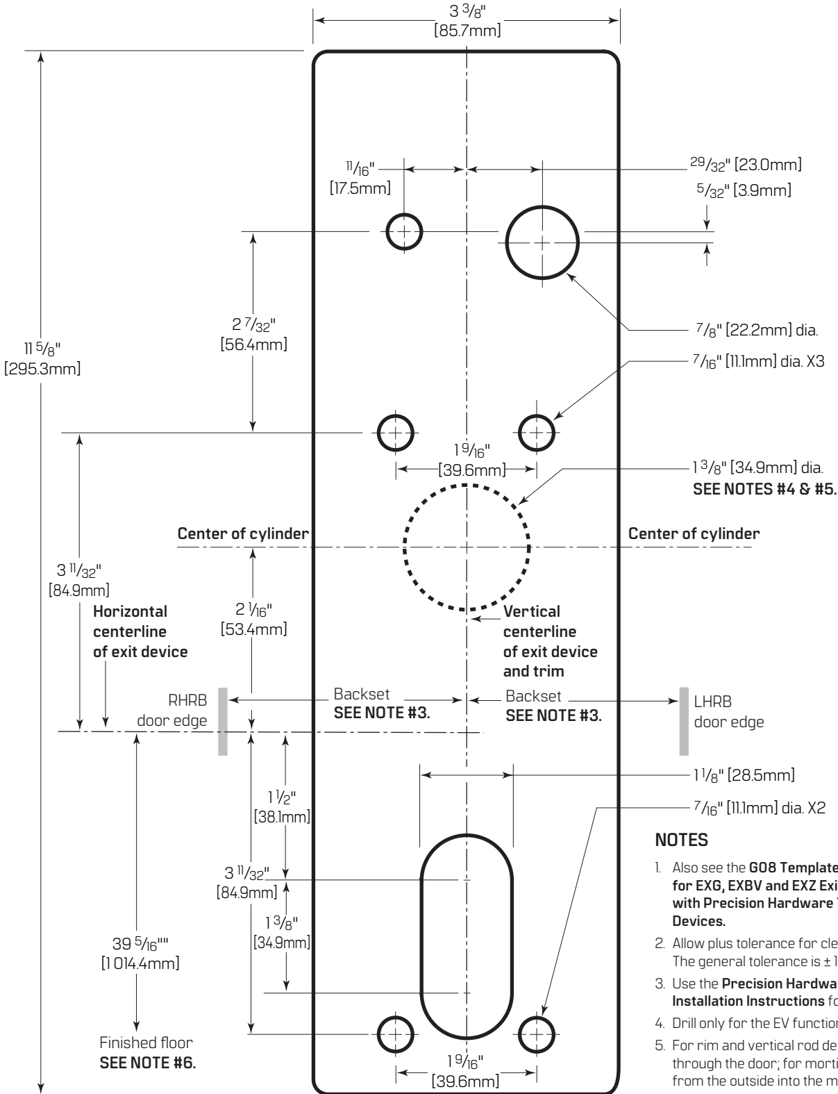
Exit Hardware Trim Escutcheon *Template not to scale
