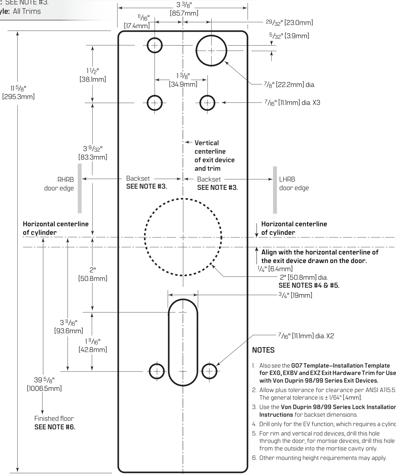
Exit Hardware Trim Escutcheon *Template not to scale
