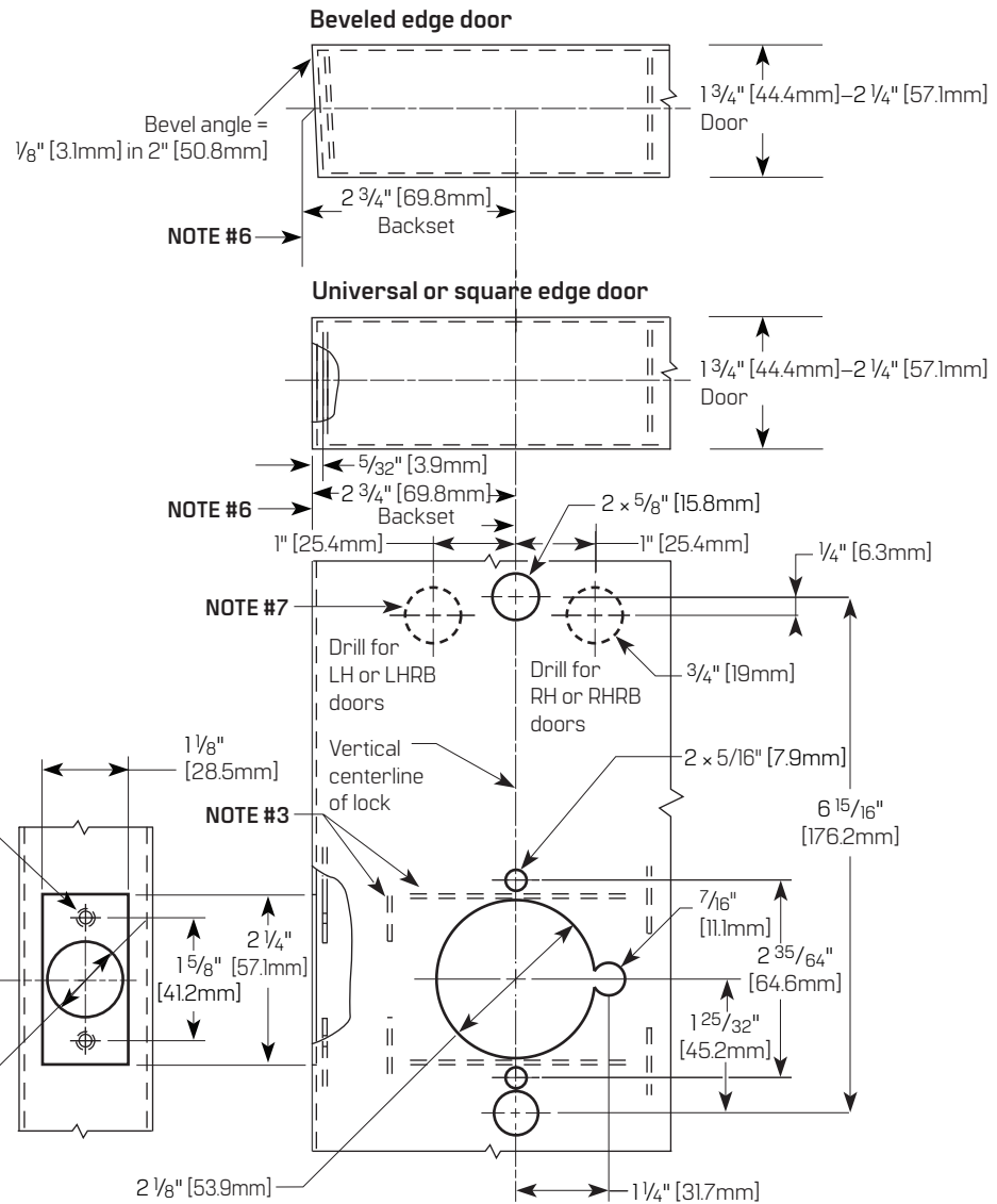
2-3/4" [69.8mm] Backset Door Preparation *Template not to scale
