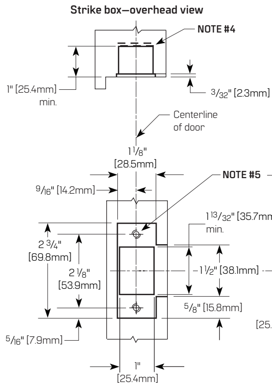
Frame Preparation *Template not to scale
