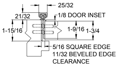
CLOSED POSITION
