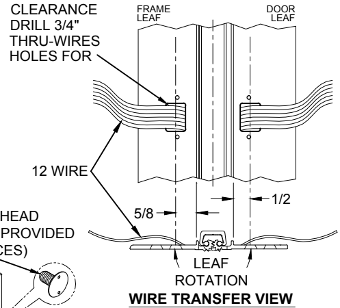
ROTATION WIRE TRANSFER VIEW
