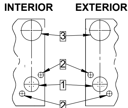
SUGGESTED DOOR CUT
