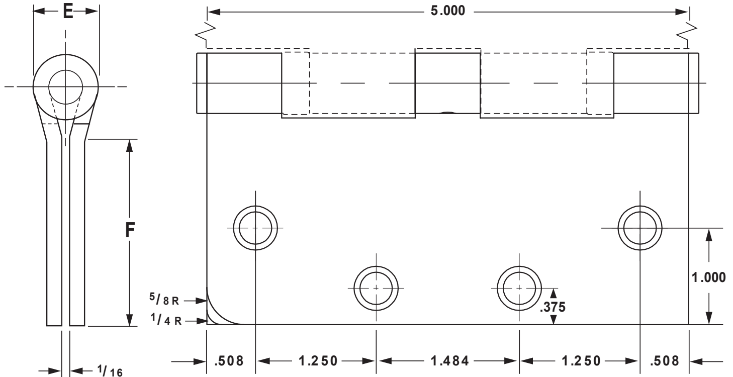
Template to scale 1 : 1, full size.
