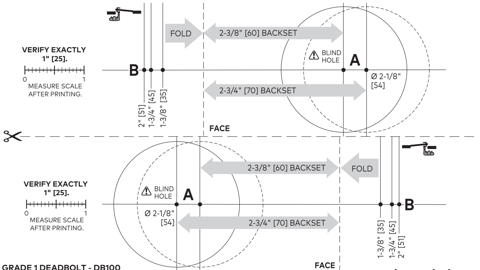
GRADE 1 DEADBOLT - DB100 INSTALLATION TEMPLATE
