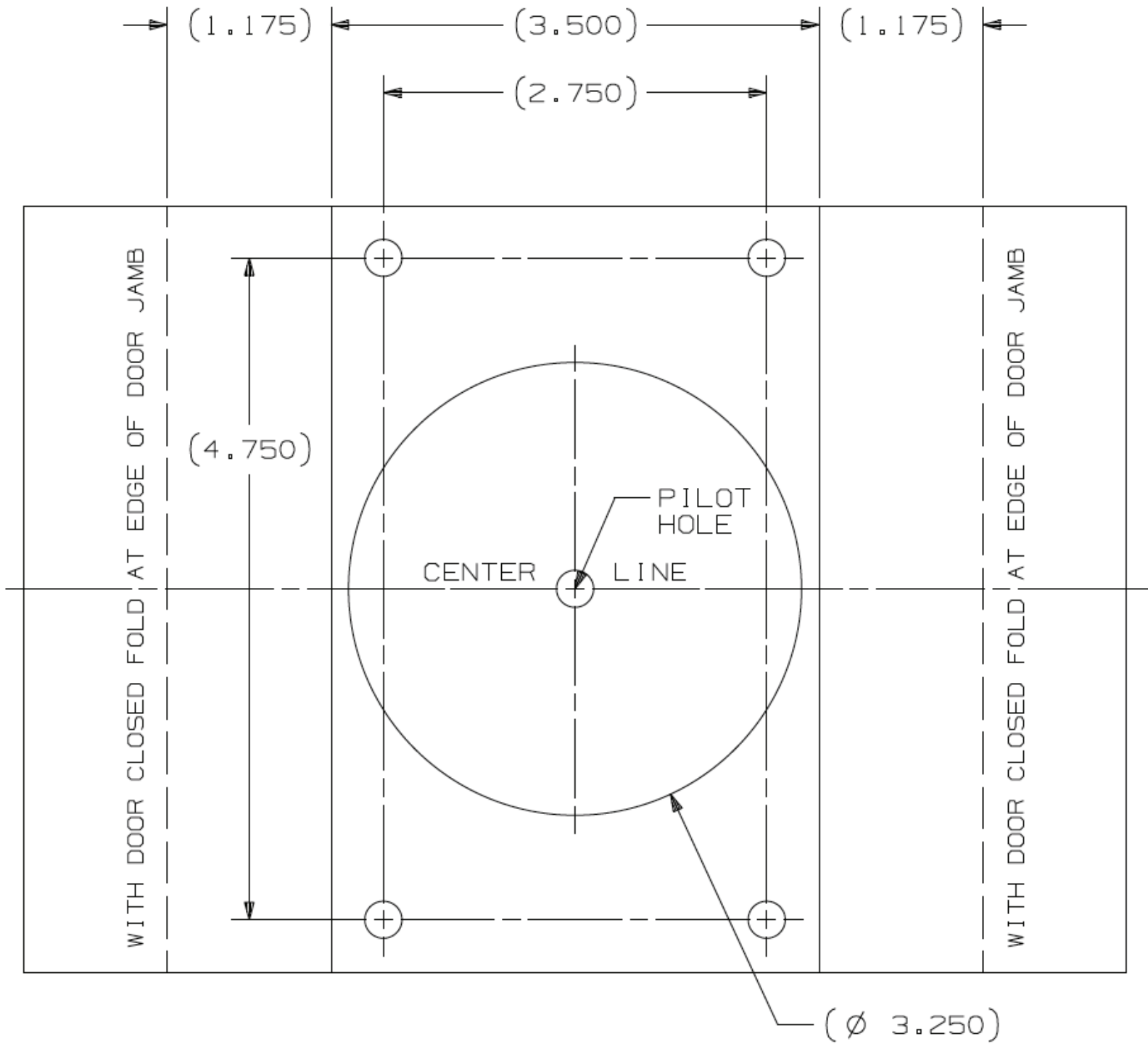
MORTISE KEEPER DRILL TEMPLATE
